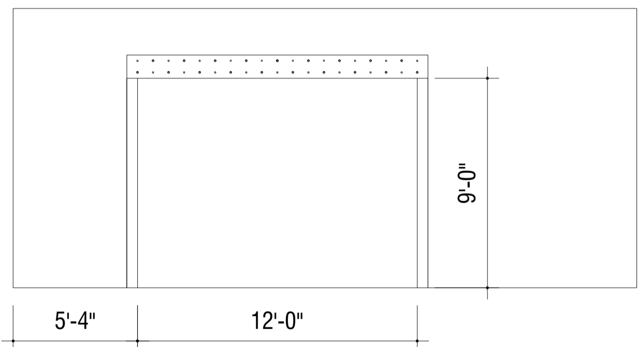
3 FRAMED OPENING DETAIL SCALE: 1/4" = 1'-0"
